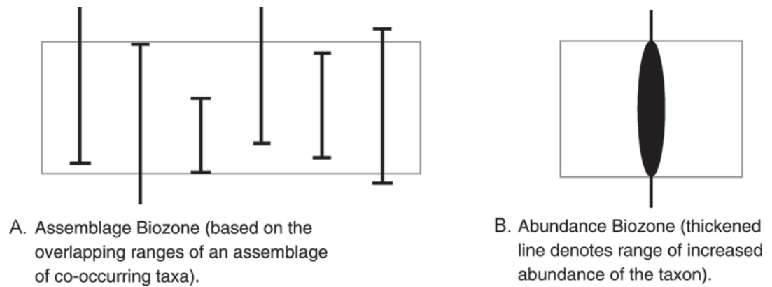
Figure 5. Examples of assemblage and abundance biozones.
