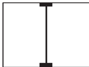
A. Taxon-range Biozone (based on the range of a taxon).
