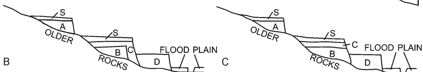
B Transverse lateral cross section of valley wall at XX' in Figure 9A
